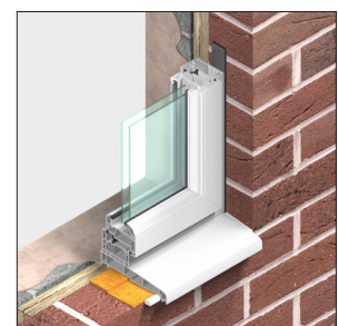
Fig. 4 TP650 installed (FM330 under sill)
